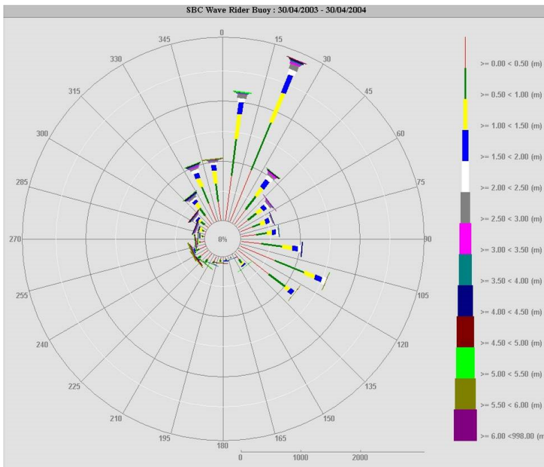
Figure 2.17 Wave Rose at Scarborough SBC site
