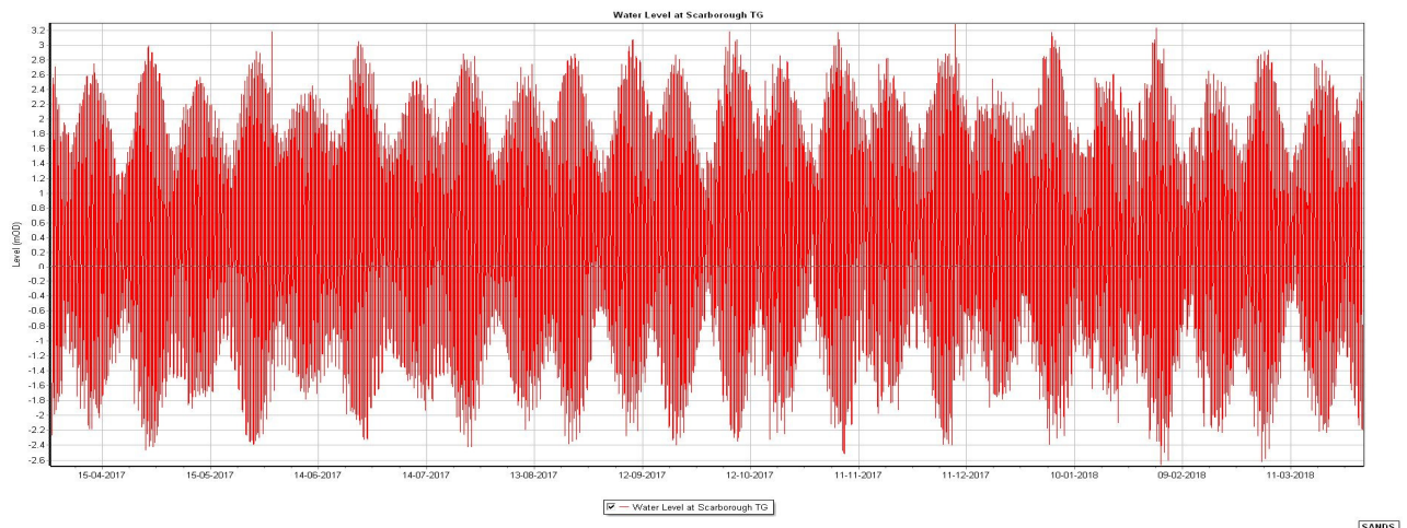
Figure 2.19 Water Levels at Scarborough TG Recorded Tide Site for 2017-18
