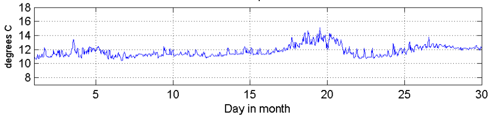
Sea temperature
