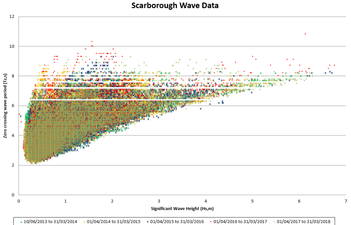
Figure 2.13 Scatter plot of Wave Height Vs Peak Period offshore Scarborough
