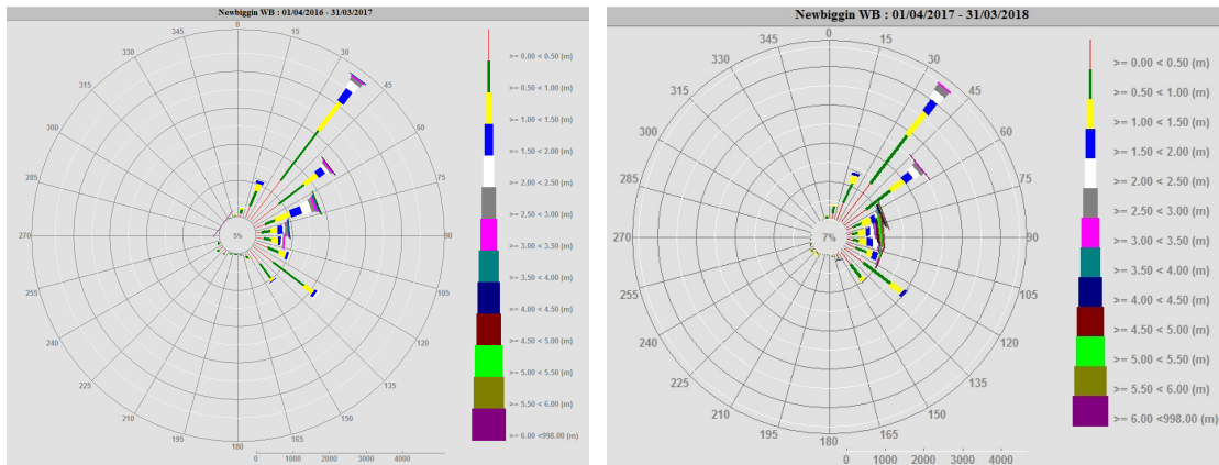
Figure 2.2 Wave roses for Newbiggin WB original deployment in 2010/11 and new data for 2013/14, 2014/15, 2015/16, 2016/17 and 2017/18
