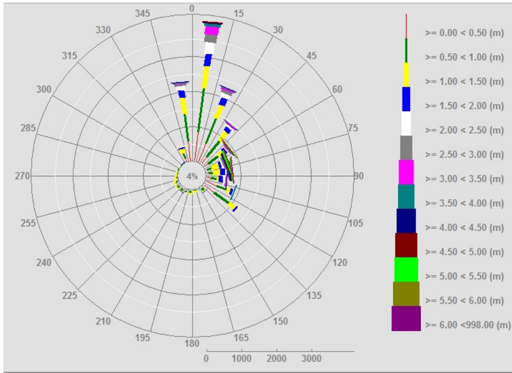
Wave Rose for Scarborough Wave Buoy 2017-18
