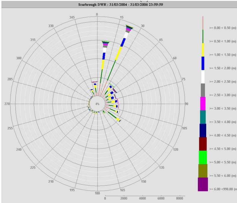
Figure 2.16 Wave Rose at Scarborough DWR site
