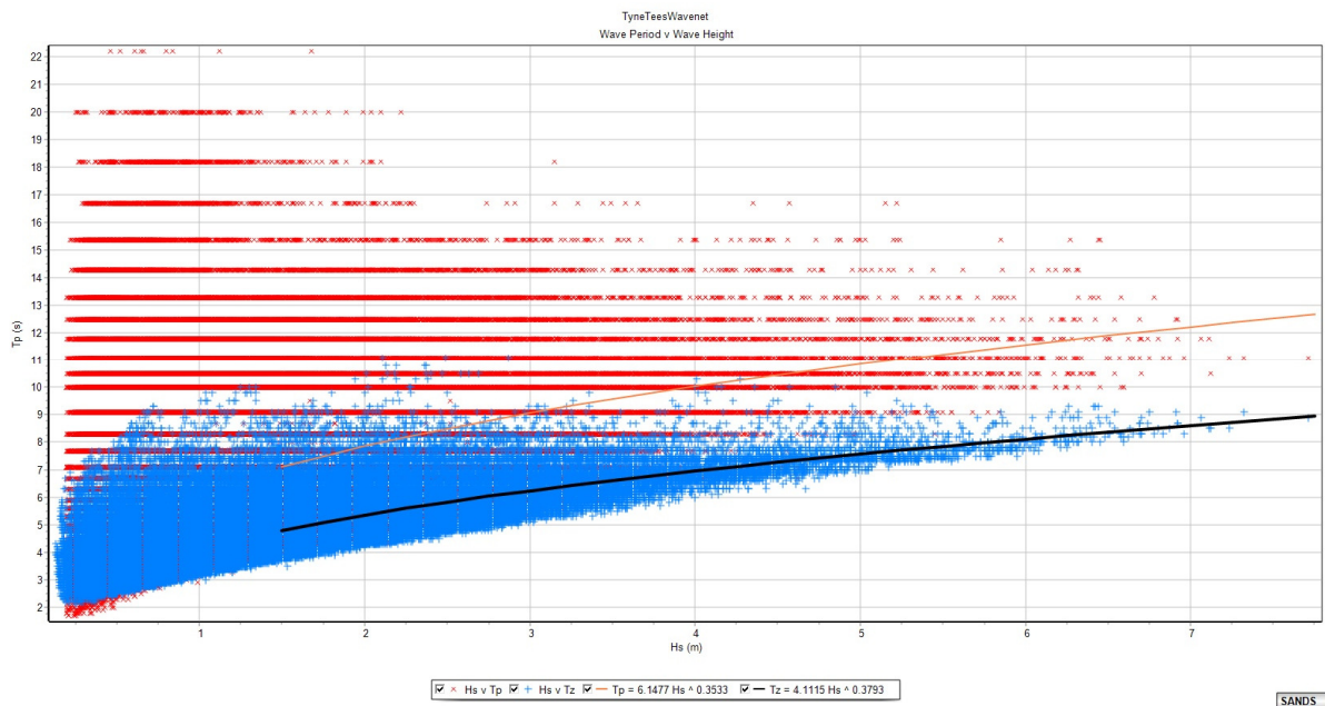
Figure 2.6 Scatter plot of Wave Height Vs Peak Period at Tyne Tees wave buoy site
