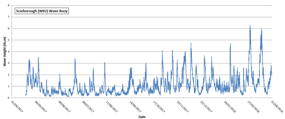
Figure 4.2 Wave height data for 2017-18 in Cell 1
