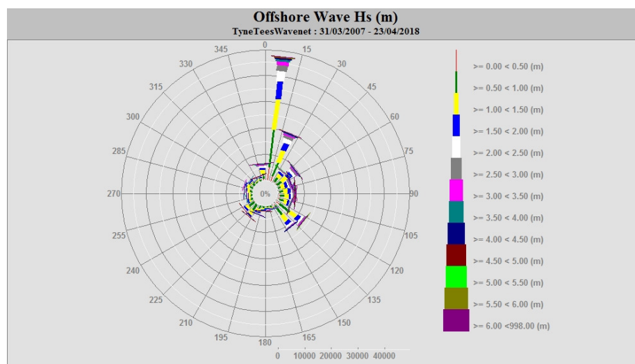
Figure 2.7 Wave Rose at Tyne Tees wave buoy site (WMO ID 62293)
