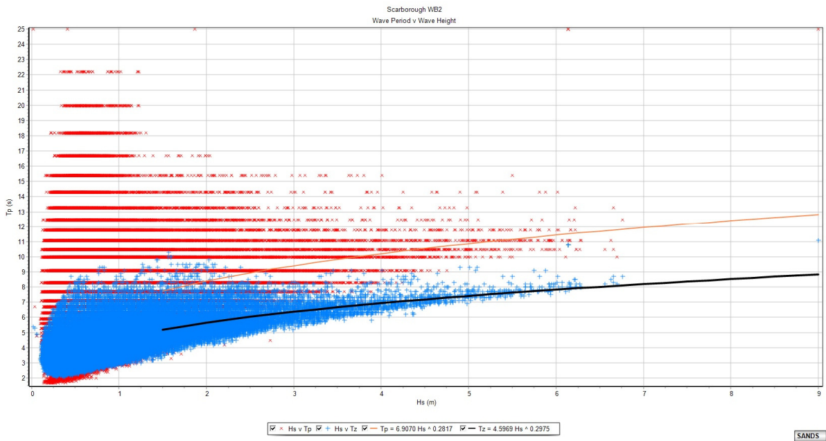
Figure 2.15 Scatter plot Wave Height Vs Period at Scarborough WB2 site (June 2013 to March 2018)
